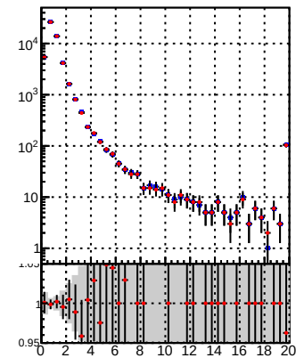
N of reco track vs. —●— DQM TT mkFit-DQM_pless_orig —●— DQM TT mkFit-DQM_pless_modi2
