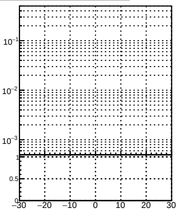
l of associated (recoToSim) loop tracks vs transverse ref point position
