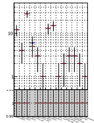
N of reco track vs. \chi^2 DQM TT mkFit-DQM_pless_orig DQM TT mkFit-DQM_pless_modi2
