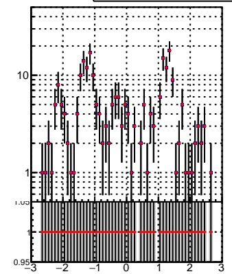
—●— DQM_TT_mkFit-DQM_pless_orig —●— DQM_TT_mkFit-DQM_pless_modi2
