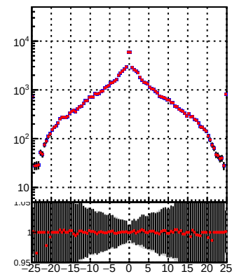
—•— DQM_TT mkFit-DQM_pless_orig —•— DQM_TT mkFit-DQM_pless_modi2
