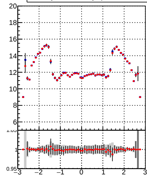
— DQM_TT_mkFit-DQM_pless_orig — DQM_TT_mkFit-DQM_pless_modi2
