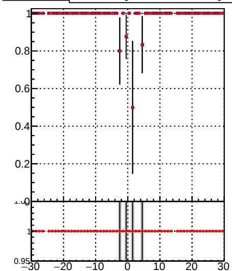
Fake rate vs vertpos Legend: DQM_TT_mkFit-DQM_pless_orig (grey line with error bars), DQM_TT_mkFit-DQM_pless_modi2 (red line with error bars)
