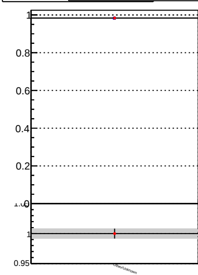
Fake rate vs. —•— DQM_TT_mkFit-DQM_pless_orig —•— DQM_TT_mkFit-DQM_pless_modi2
