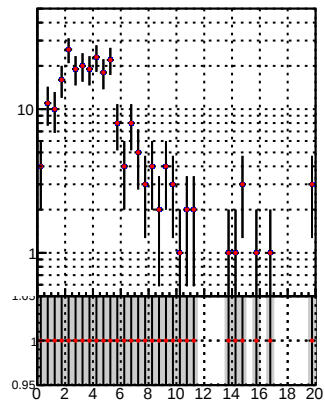
N of reco track vs. \chi^2 for DQM TT mkFit-DQM_pless_orig and DQM TT mkFit-DQM_pless_mod12
