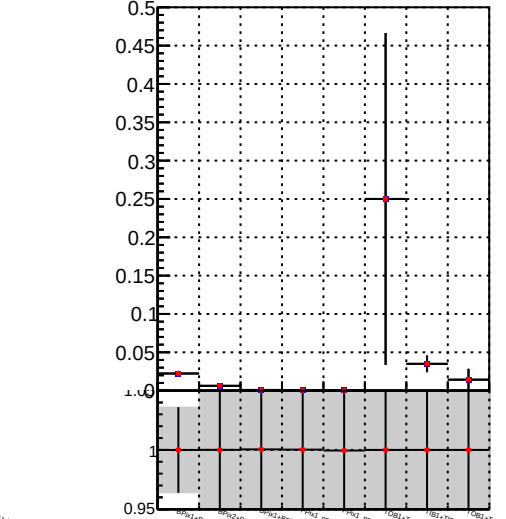
Fake rate vs. —●— DQM TT mkFit-DQM_pless_orig —●— DQM TT mkFit-DQM_pless_modi2
