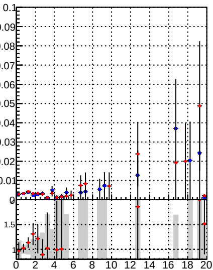
Duplicates Rate vs normalized \chi^2
