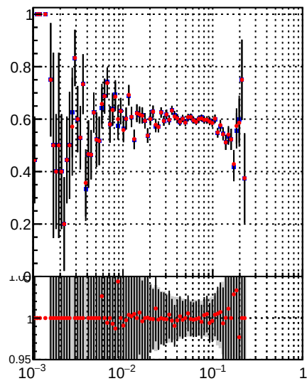
—•— DQM_TT_mkFit-DQM_pless_orig —•— DQM_TT_mkFit-DQM_pless_modi2
