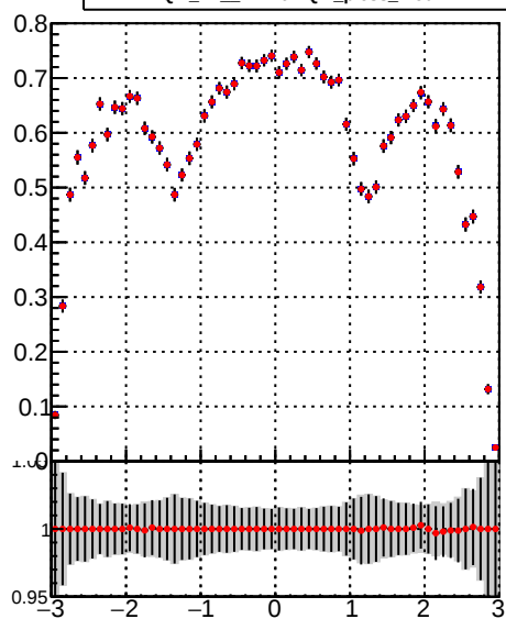
—•— DQM_TT_mkFit-DQM_pless_orig —•— DQM_TT_mkFit-DQM_pless_modi
