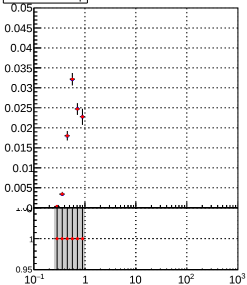
Legend: DQM_TT_mkFit-DQM_pless_orig DQM_TT_mkFit-DQM_pless_modi
