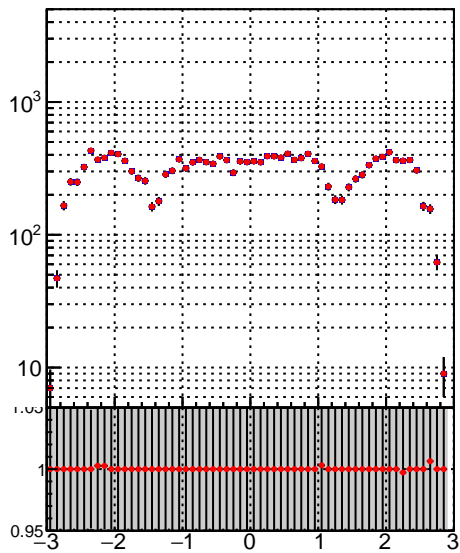
■ DQM_TT_mkFit-DQM_pless_orig ● DQM_TT_mkFit-DQM_pless_modi
