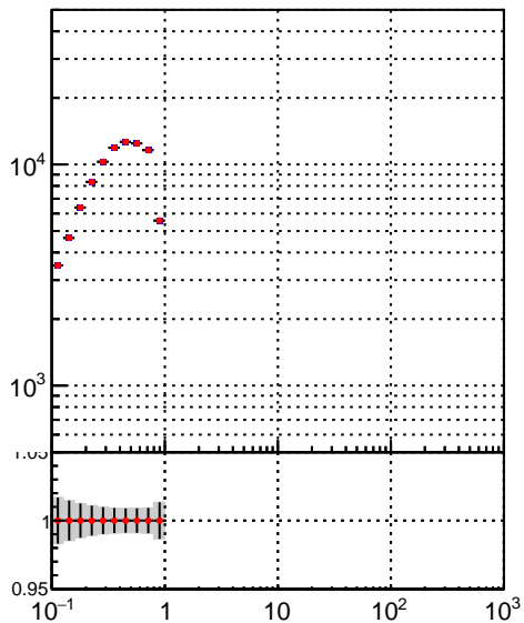
■ DQM_TT_mkFit-DQM_pless_orig ● DQM_TT_mkFit-DQM_pless_modi
