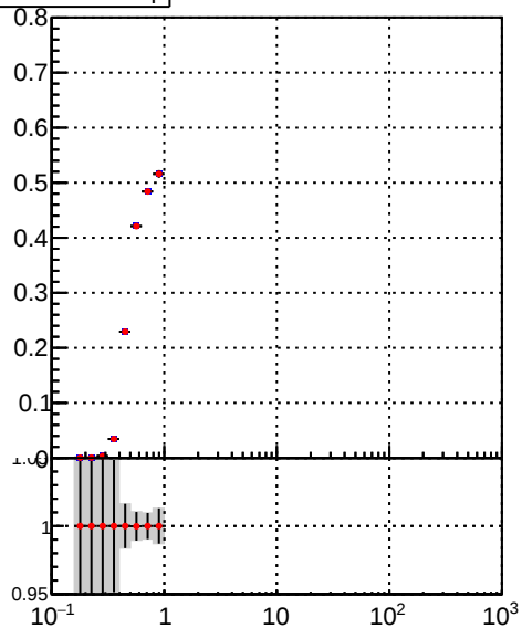
DQM_TT_mkFit-DQM_pless_orig DQM_TT_mkFit-DQM_pless_modi
