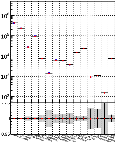
Number of tracks vs collection
