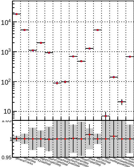
Number —●— DQM_TT_mkFit-DQM_pless_modi
