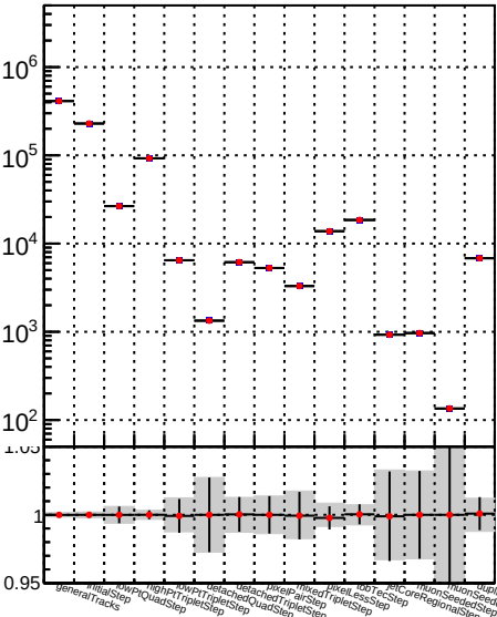
Number of true tracks vs collection
