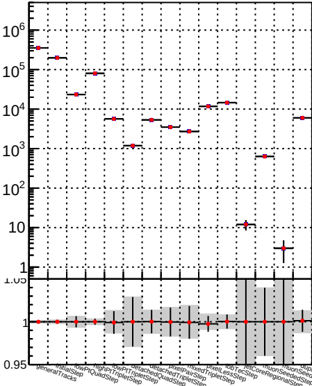
Number of pileup tracks vs collection
