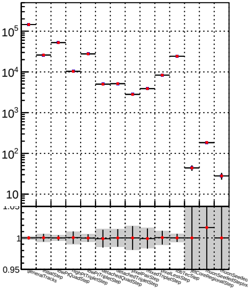
Number —●— DQM_TT__mkFit-DQM_pless_modi
