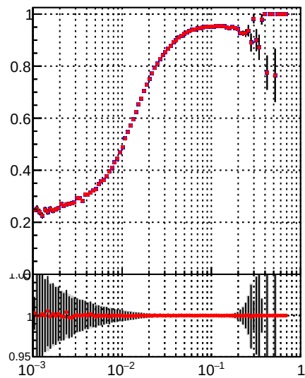
—•— DQM_TT_mkFit-DQM_pless_orig —•— DQM_TT_mkFit-DQM_pless_modi
