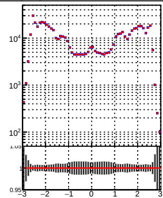
DQM_TT_mkFit-DQM_pless_orig DQM_TT_mkFit-DQM_pless_modi
