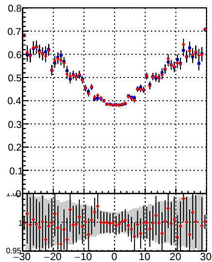
Fake rate vs d —•— DQM_TT_mkFit-DQM_pless_orig —•— DQM_TT_mkFit-DQM_pless_modi
