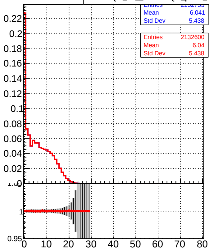
—■— DQM_TT_mkFit-DQM_pless_orig —●— DQM_TT_mkFit-DQM_pless_modi
