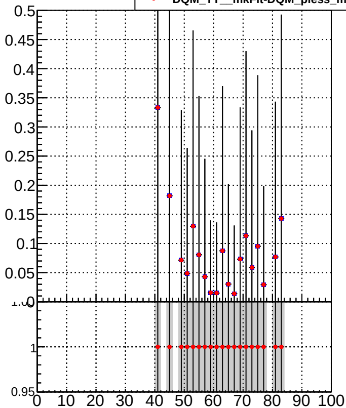
■ DQM_TT_mkFit-DQM_pless_orig ● DQM_TT_mkFit-DQM_pless_modi
