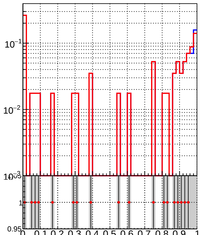
RecoPVAssoc2GenPVNotMatched_Purity
