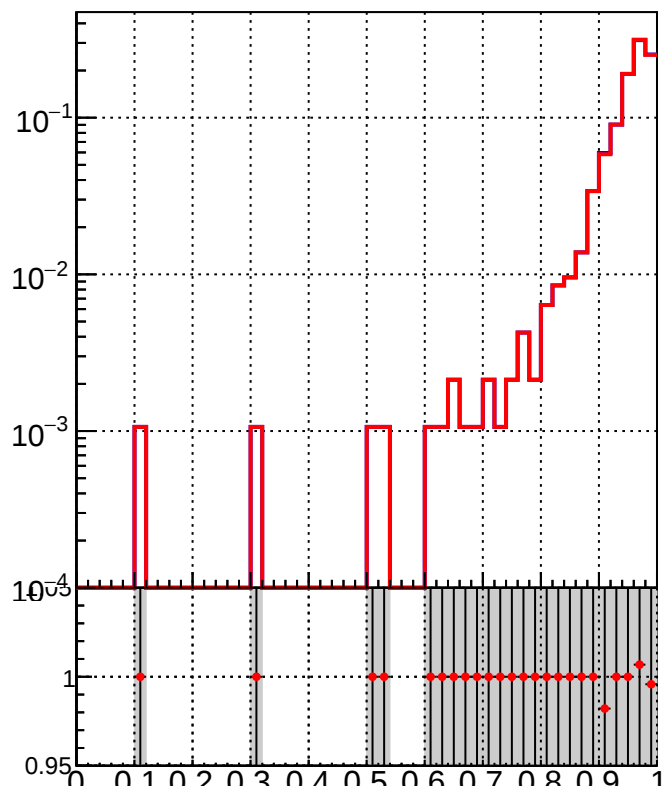
RecoPVAssoc2GenPVMatched_Purity
