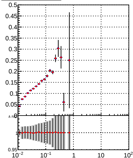
—•— DQM_TT_mkFit-DQM_pless_orig —•— DQM_TT_mkFit-DQM_pless_modi
