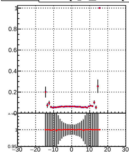
—•— DQM_TT_mkFit-DQM_pless_orig —•— DQM_TT_mkFit-DQM_pless_modi
