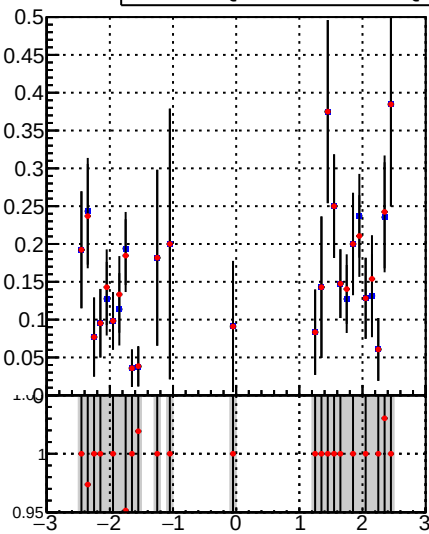
—■— DQM_TT_mkFit-DQM_pless_orig —●— DQM_TT_mkFit-DQM_pless_modi
