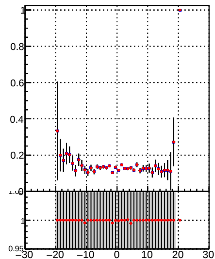
Fake rate vs d —•— DQM TT mkFit-DQM_pless_orig —•— DQM TT mkFit-DQM_pless_modi
