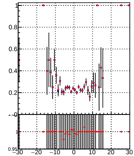
—•— DQM_TT_mkFit-DQM_pless_orig —•— DQM_TT_mkFit-DQM_pless_modi
