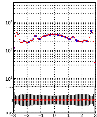
N of reco track vs \eta pT eta —•— DQM_TT_mkFit-DQM_pless_orig —•— DQM_TT_mkFit-DQM_pless_modi
