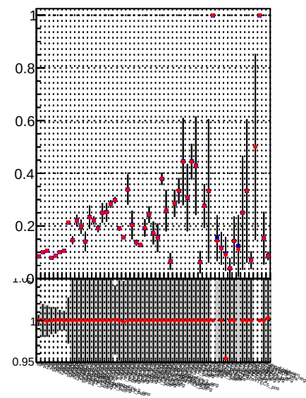
Fake rate vs. Legend for the bottom row of plots: —•— DQM TT mkFit-DQM_pless_orig —•— DQM TT mkFit-DQM_pless_modi
