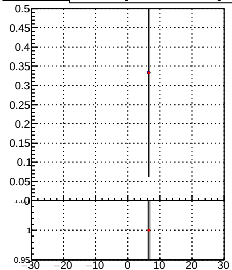
Fake rate vs vertpos Legend: DQM_TT_mkFit-DQM_pless_orig (grey shaded), DQM_TT_mkFit-DQM_pless_modi (red dot)
