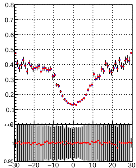
—•— DQM_TT_mkFit-DQM_pless_orig —•— DQM_TT_mkFit-DQM_pless_modi
