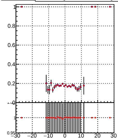
—•— DQM_TT_mkFit-DQM_pless_orig —•— DQM_TT_mkFit-DQM_pless_modi
