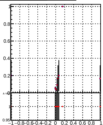
DQM_TT_mkFit-DQM_pless_modi
