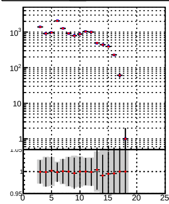
—•— DQM_TT_mkFit-DQM_pless_orig —•— DQM_TT_mkFit-DQM_pless_modi
