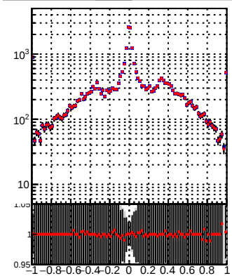
—•— DQM_TT_mkFit-DQM_pless_orig —•— DQM_TT_mkFit-DQM_pless_modi
