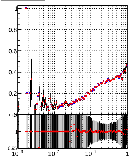
Fake rate vs \sqrt{s} Legend: DQM_TT_mkFit-DQM_pless_orig (black line with error bars) DQM_TT_mkFit-DQM_pless_modi (red line with error bars)
