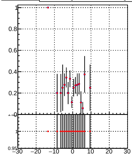
Fake rate vs v Legend: DQM_TT_mkFit-DQM_pless_orig DQM_TT_mkFit-DQM_pless_modi
