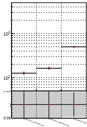
N of reco track vs. \chi^2 —•— DQM TT mkFit-DQM_pless_orig —•— DQM TT mkFit-DQM_pless_modi
