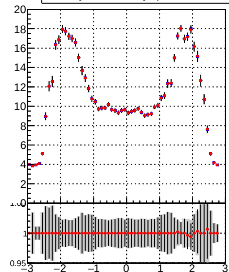
mean hit — DQM_TT_mkFit-DQM_pless_orig — DQM_TT_mkFit-DQM_pless_modi
