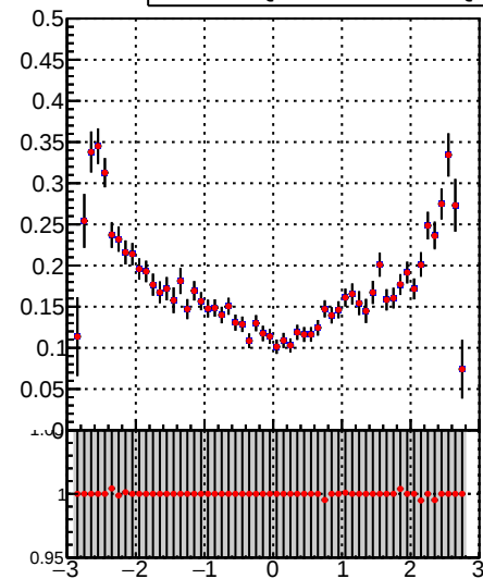
■ — ● DQM_TT_mkFit-DQM_pless_orig — ● DQM_TT_mkFit-DQM_pless_modi
