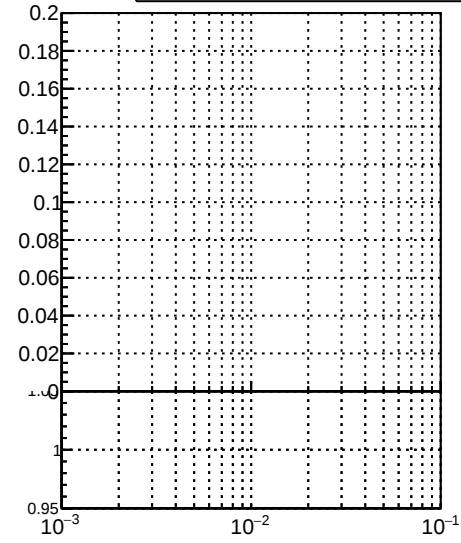
Fake rate vs \sqrt{s} DQM_TT_mkFit-DQM_pless_orig DQM_TT_mkFit-DQM_pless_modi
