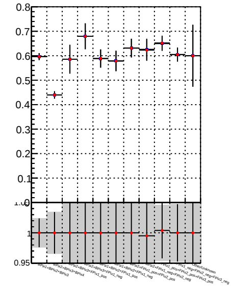
Fake rate vs. DQM_TT_mkFit-DQM_pless_orig DQM_TT_mkFit-DQM_pless_modi
