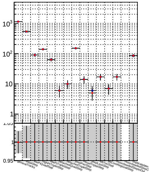
Number —●— DQM_TT__mkFit-DQM_pless_modi
