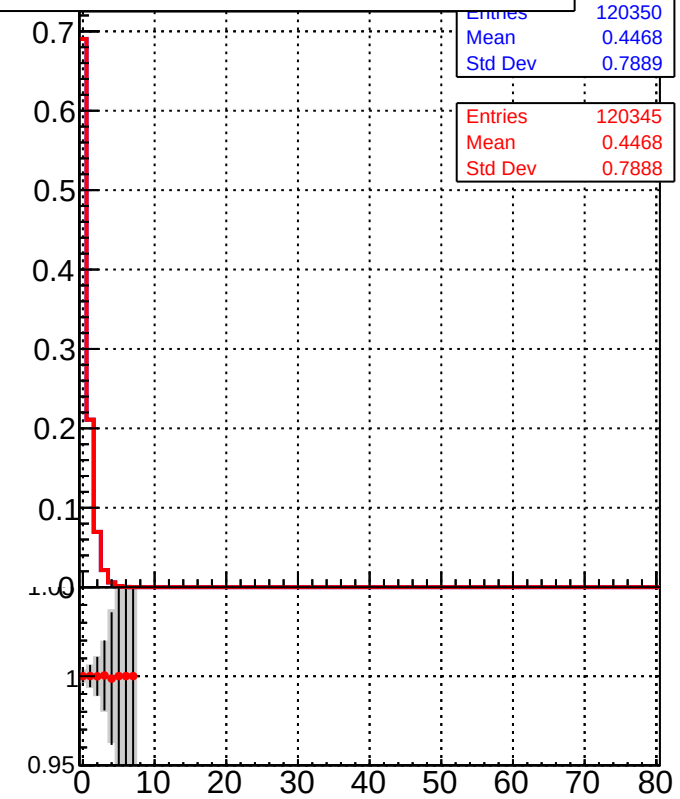
Legend: DQM_TT_mkFit-DQM_pless_orig (grey histogram), DQM_TT_mkFit-DQM_pless_modi (red line with markers)
