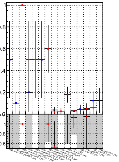
Fake rate vs. DQM TT mkFit-DQM_pless_orig DQM TT mkFit-DQM_pless_modi
