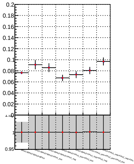
Fake rate vs. DQM_TT_mkFit-DQM_pless_orig DQM_TT_mkFit-DQM_pless_modi
