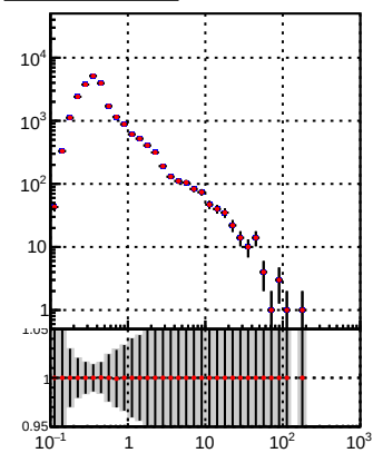
—•— DQM_TT_mkFit-DQM_pless_orig —•— DQM_TT_mkFit-DQM_pless_modi
