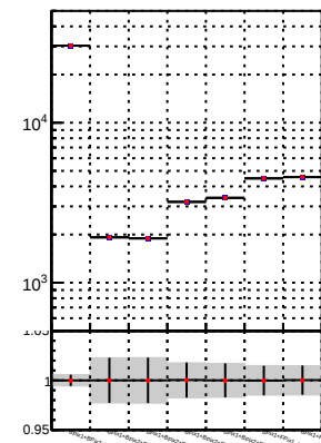
N of reco track vs. \chi^2 — DQM TT mkFit-DQM_pless_orig — DQM TT mkFit-DQM_pless_modi
