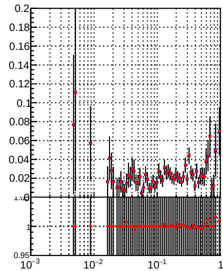
Fake rate vs \sqrt{s} DQM_TT_mkFit-DQM_pless_orig DQM_TT_mkFit-DQM_pless_modi
